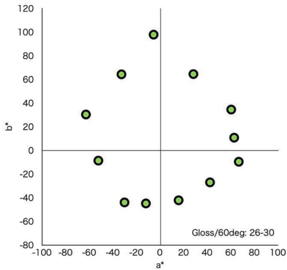
Figure 10. Laser Matte Mode Printing Gamut (matte paper)
