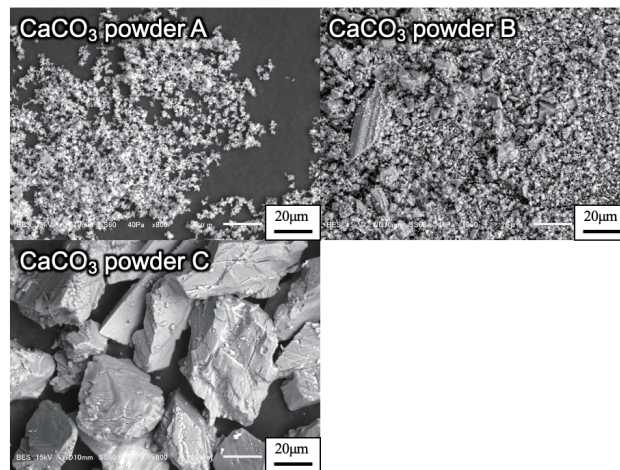
Figure 4. The powders used in this study are composed of calcium carbonate. Powders A and B possess fine particle sizes on the order of a few micrometers; powder A corresponds to light calcium carbonate, while powders B and C represent heavy calcium carbonate. Powder C has a relatively large particle size of several tens of micrometers.
