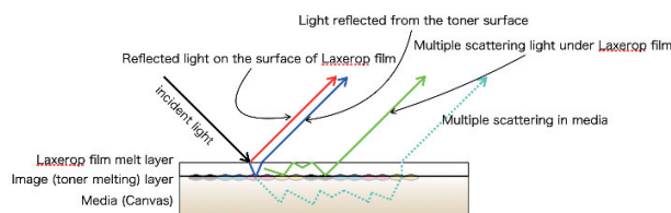
Figure 7. Principles of Laxerop Canvas
