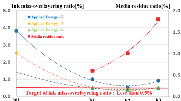
Figure 3 : Ink miss-over-layering and media residue ratio by height of heater element
