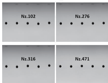
Figure 8. Droplet velocity uniformity of the 512Nz printhead
