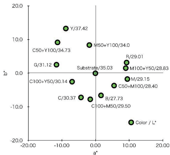
Figure 3. Laxerop Glass Printing Gamut (Reflection)
