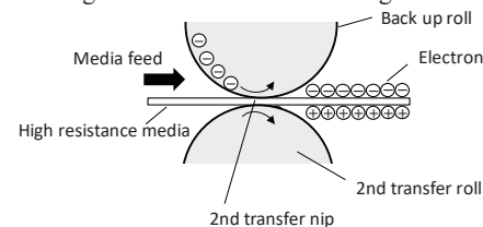
Fig.3 2nd transfer process.
