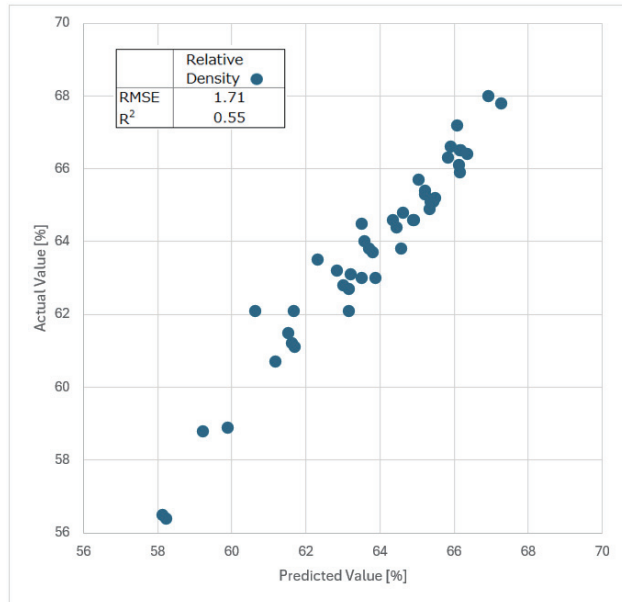
Figure 6. Prediction Results and Accuracy for Relative Density
