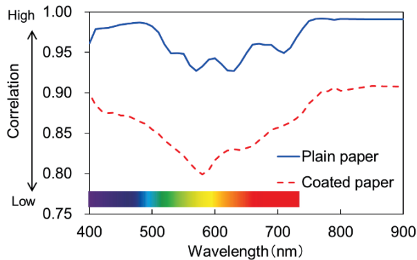
Figure 1. Correlation between transmittance and basis weight at each wavelength. [1]
