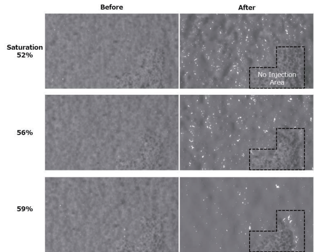
Figure 5. Photographs of the powder bed before and after heating
