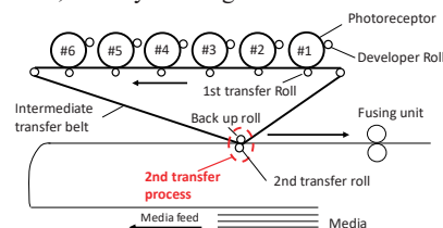
Fig.2 Electrophotographic process.
