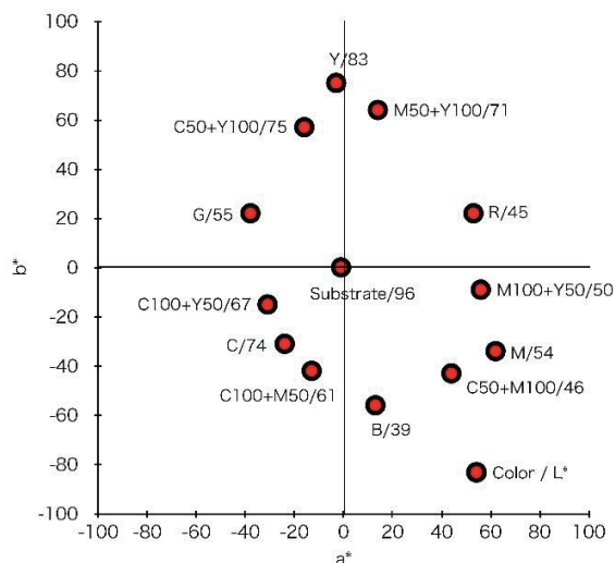
Figure 4. Laxerop Glass Printing Gamut (Transparent)
