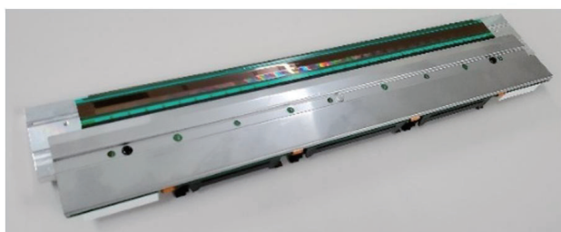
Figure 1 : New developed thermal printhead 12-inch, 1200dpi
