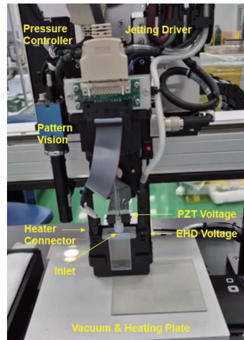
Figure 2. EHDison-H16 Printer for R&D Printing
