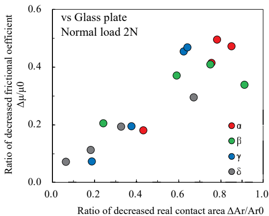
Figure 7. Relationship between the decrease ratio of the frictional force and real contact area
