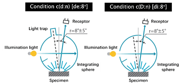
Figure 3. Diffused illumination integrating sphere system SCE (de: 8°) and SCI (di: 8°)
