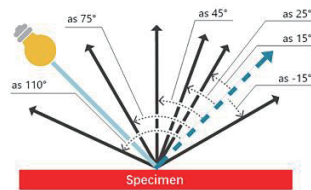
Picture 5. Multi-angle spectrophotometer CM-M6
