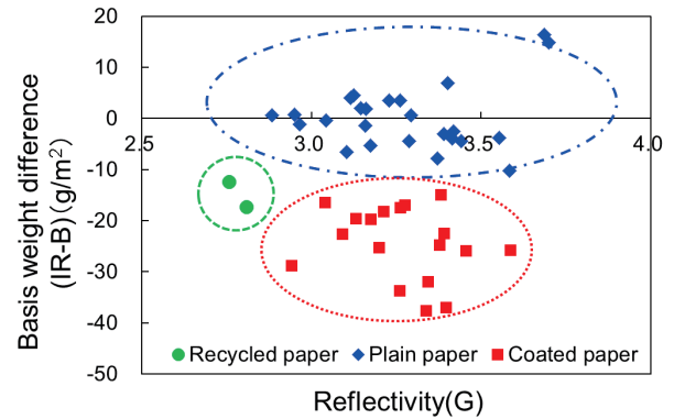
Figure 2. Classification of measured values of basis weights by paper type based on combinations of transmittance and reflectance of multiple wavelengths. [1][2]
