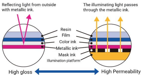
Figure 10. The mechanism of stealth printing.
