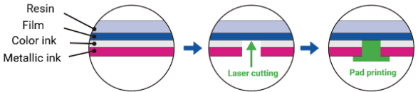
Figure 12. The process of decorative molding products using laser cutting and pad printing.
