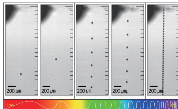
Figure 4. Droplet Ejection Results by Frequency
