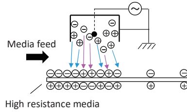
Fig. 10 Non-contact-type static eliminator.
