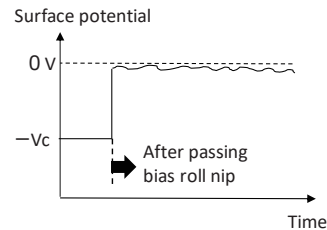
Fig. 7 Media surface potential after contact-type static eliminator.
