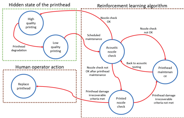
Figure 5. Reinforcement Learning based printing system controller.
