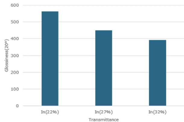
Figure 7. Transmittance and glossiness of ink ribbons.
