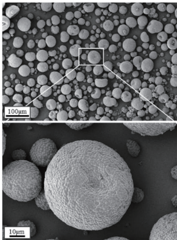
Figure 2. SEM images of granulated particle
