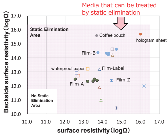
Fig.17 Media resistivity map.
